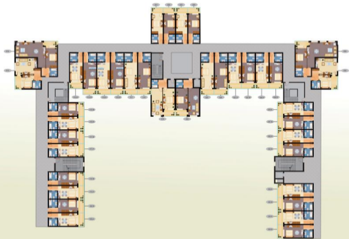
Block C, D 3rd floor
